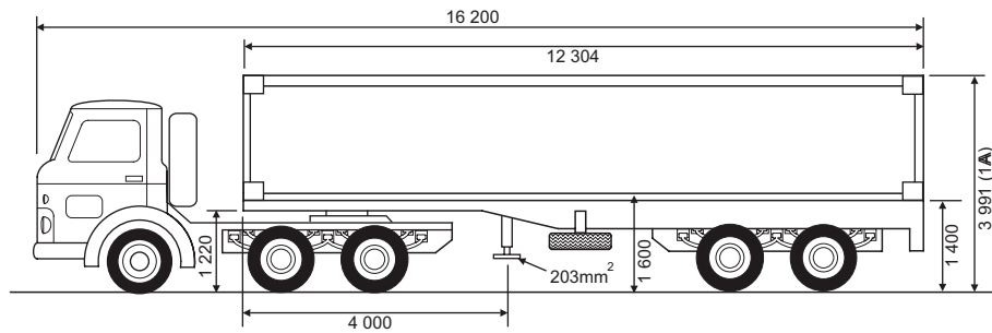
12m Skeletal Semi-trailer
