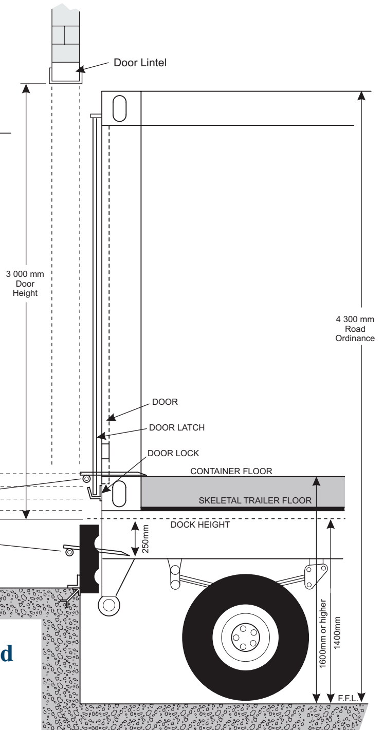
12m Skeletal Semi-trailer
