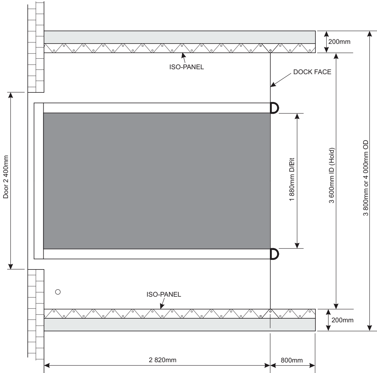
PLAN VIEW
