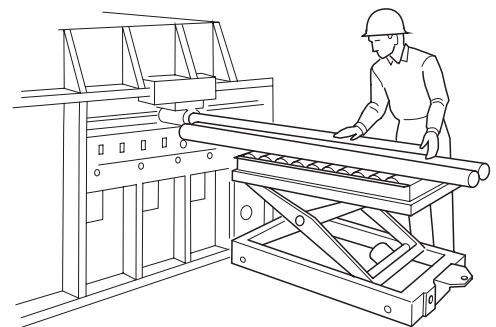
Roller Top Feeding for Cut-off Operations
