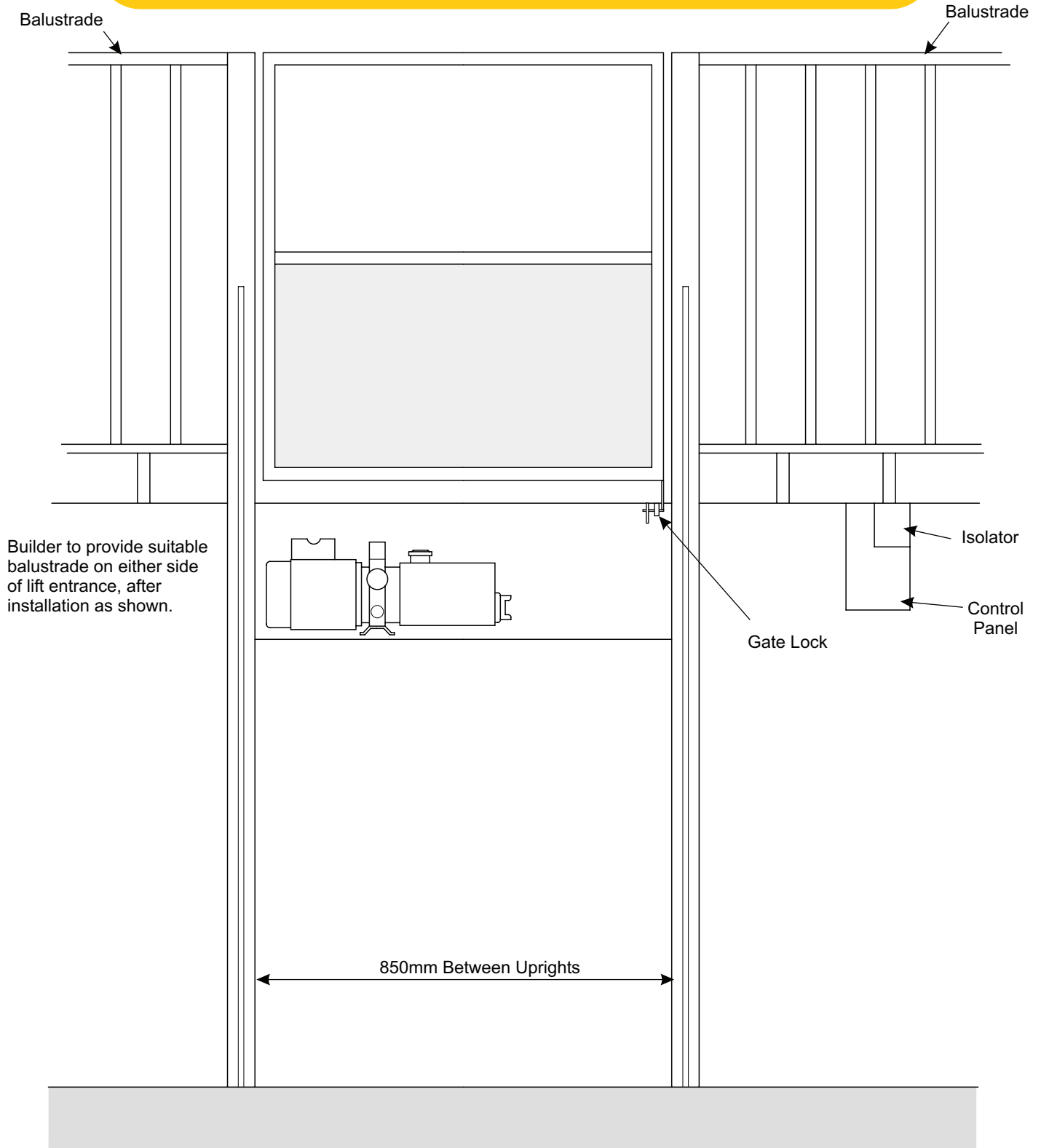
FRONT VIEW
