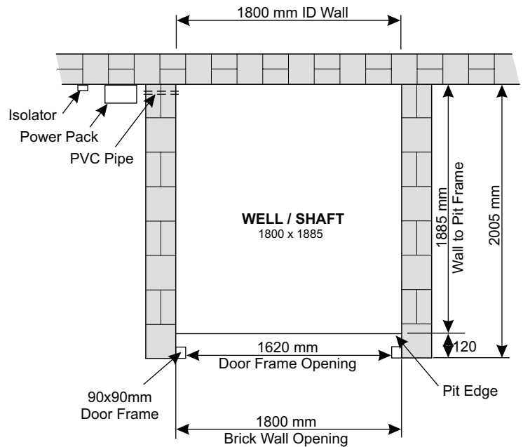
SINGLE WELL DESIGN SHAFT
