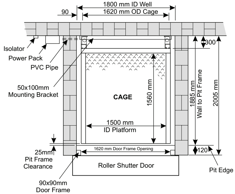
SINGLE CAGE DESIGN
