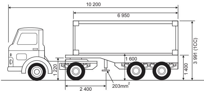
6m Skeletal Semi-trailer
