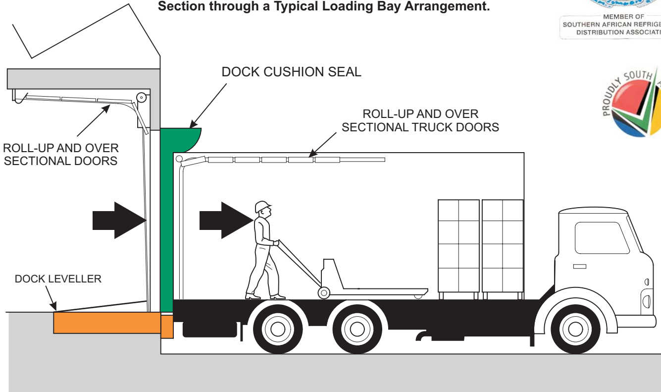
Section through a Typical Loading Bay Arrangement.
