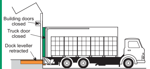
SECURE AND READY FOR DESPATCH
