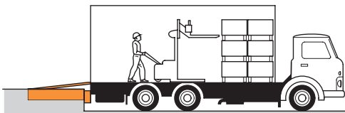
WALKIE STACKER UNLOADING 1 Man @ ½ Hour = ½ Man Hours
