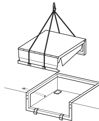
FIGURE 3b Via Overhead Crane
