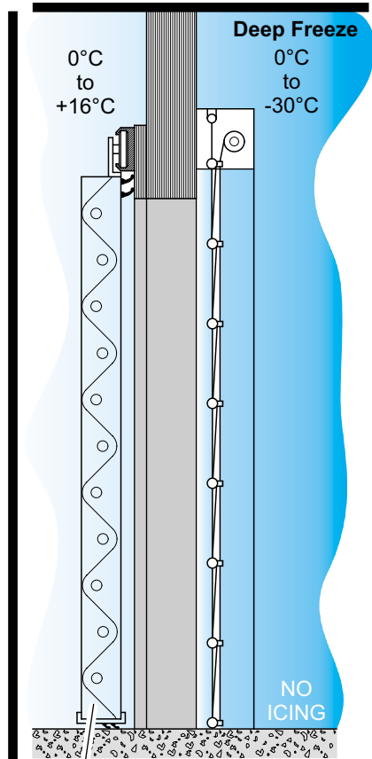
VERTICAL FOLD-UP
