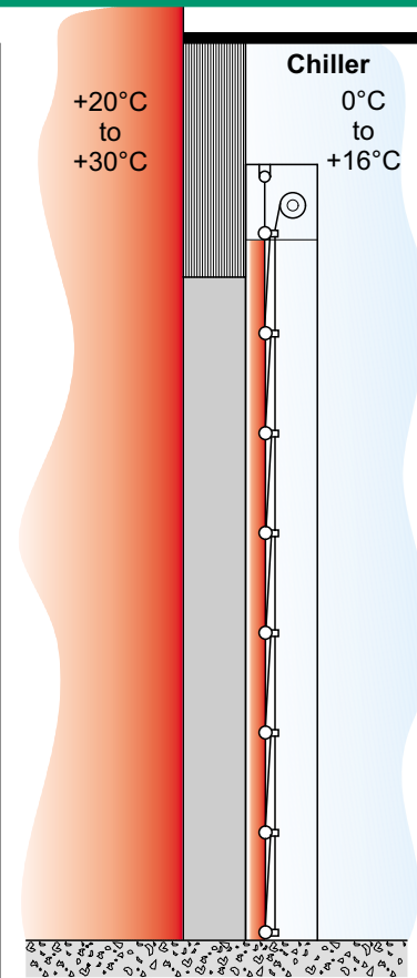
VERTICAL FOLD-UP
