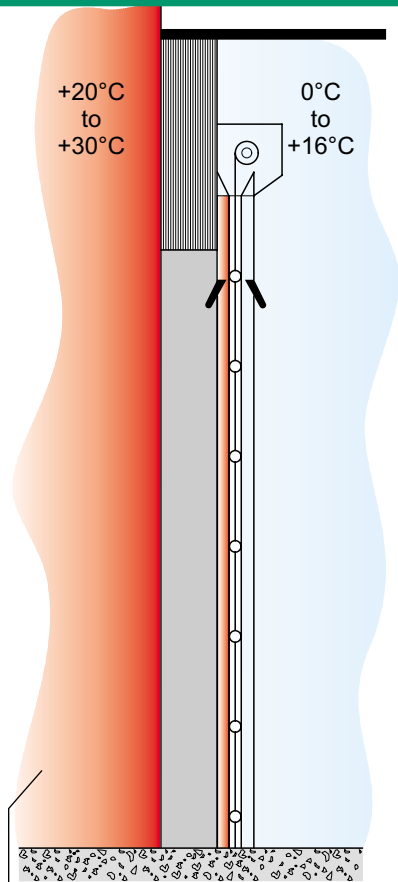
VERTICAL ROLL-UP
