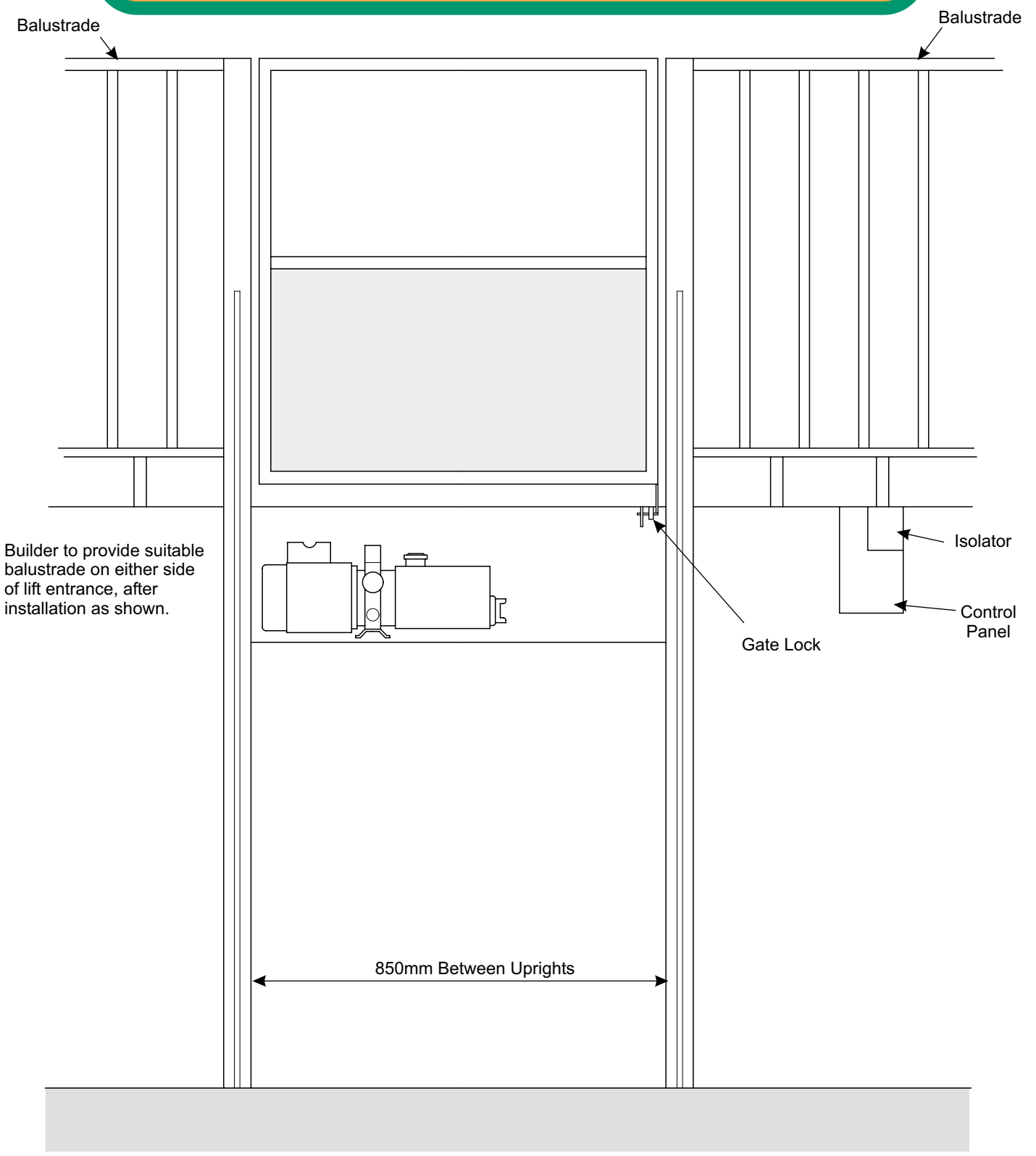
FRONT VIEW
