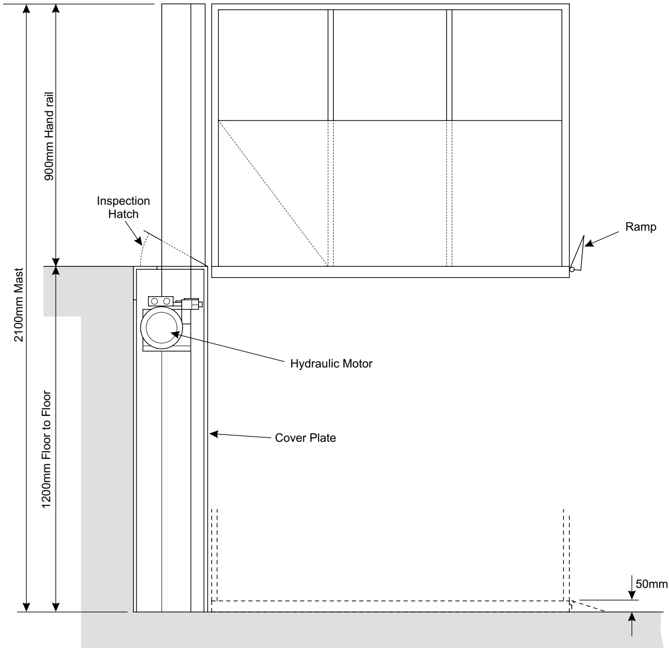
SIDE VIEW
