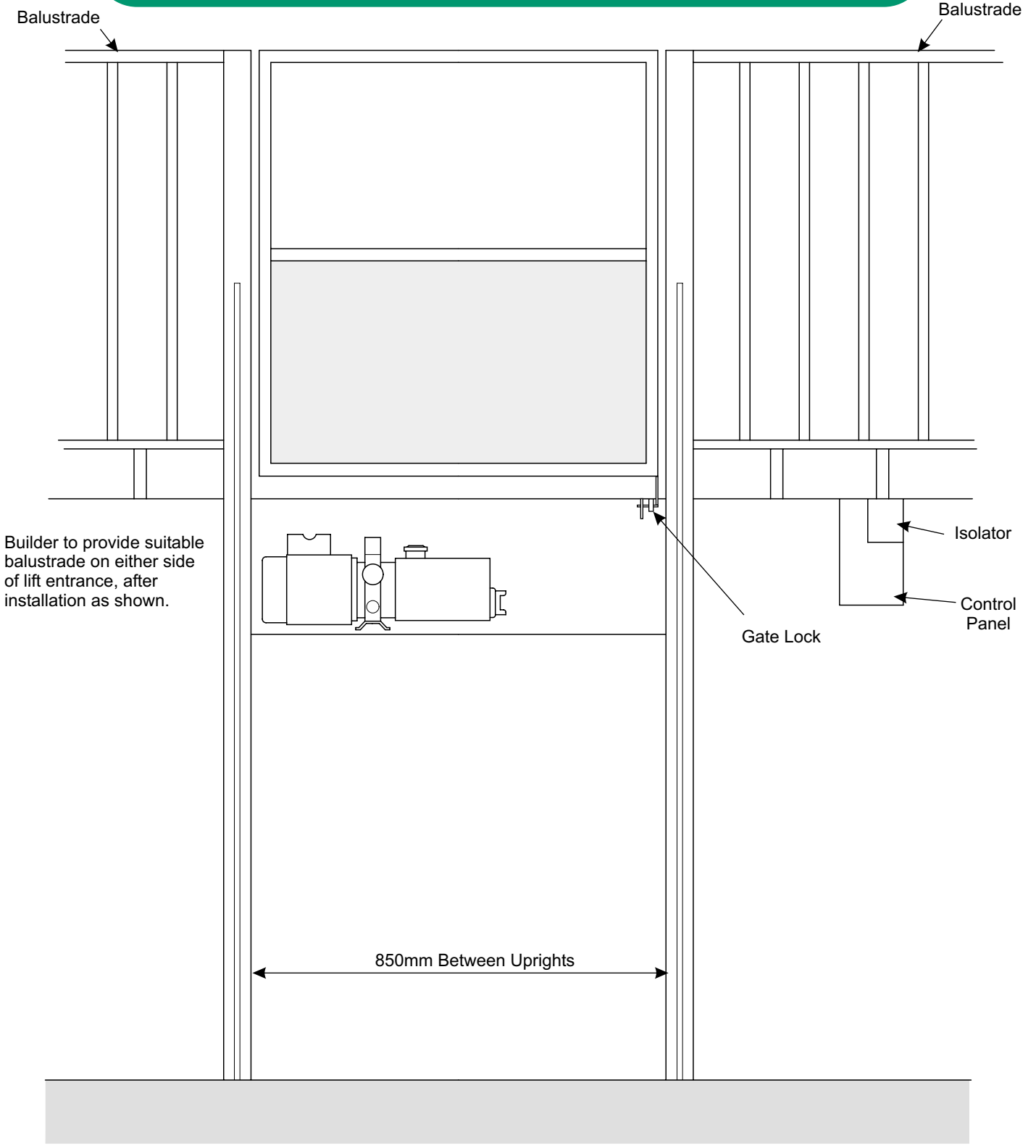
FRONT VIEW
